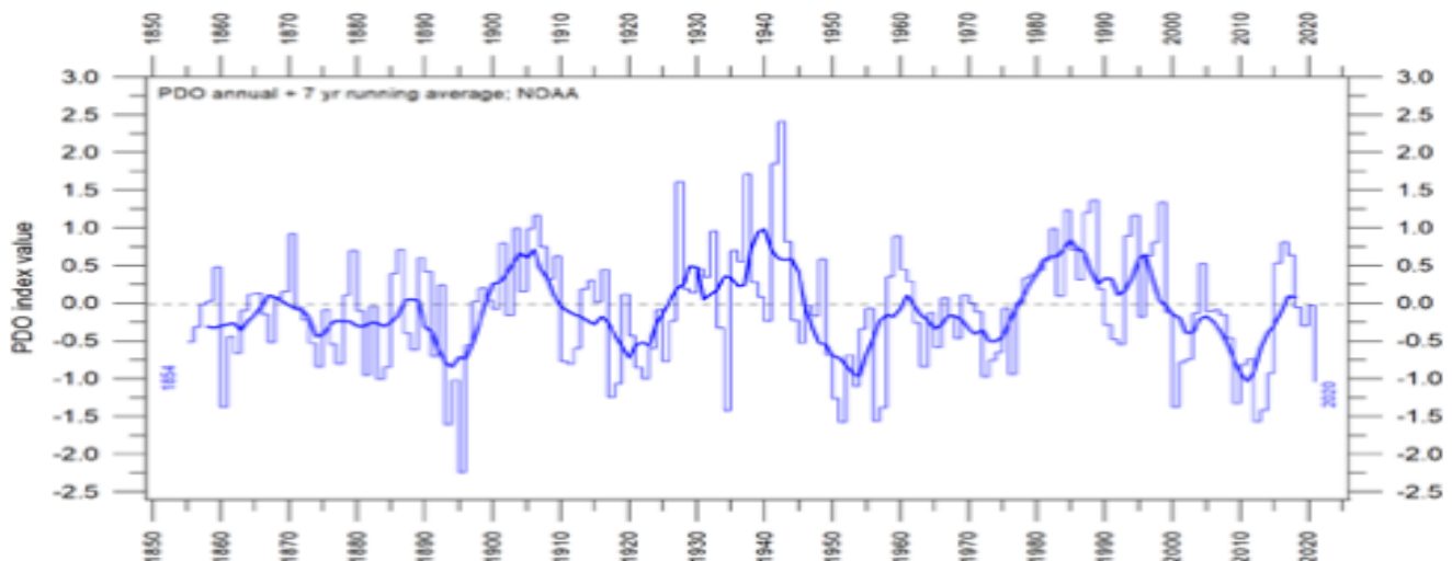
Figure 14b: Annual values 1855-2020 of the Pacific Decadal Oscillation (PDO) from Humlum 2020 According to the Physical Sciences Laboratory, NOAA. This shows the annual PDO values, the thick line is the 7-year average trend.
