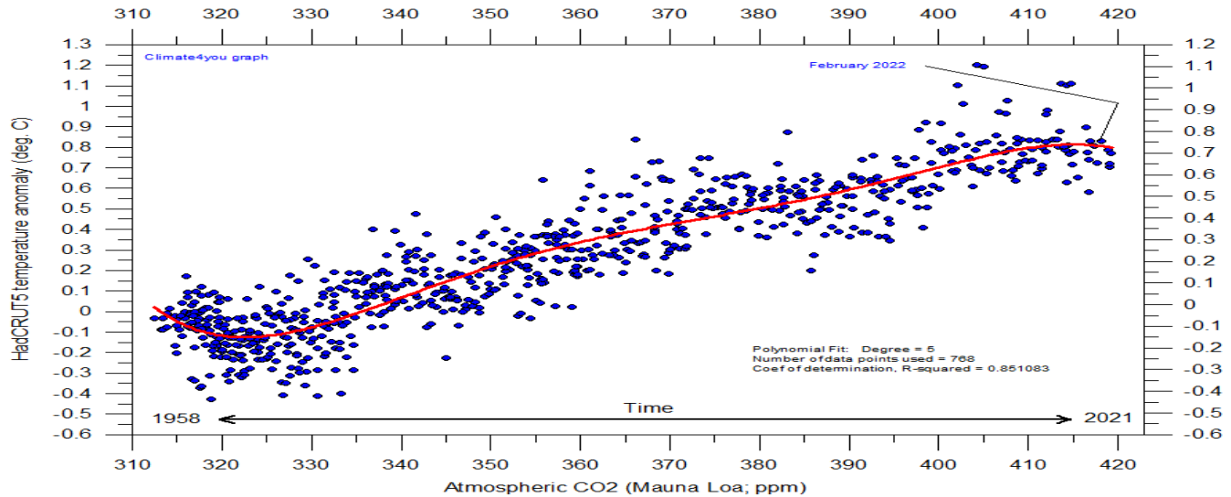
Figure 5c. HadCRUT5 monthly global surface temperature estimates versus the monthly Moana Loa atmospheric CO 2 content, after Humlum 2022 - Climate4you.com.
