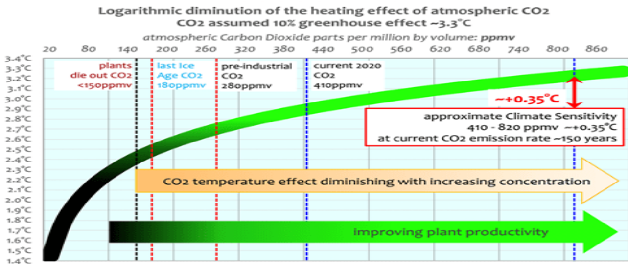
Figure 11a. A direct estimate of Climate Sensitivity to \text{CO}_2 -ECS. (after Rotter 2021 in Fabius Maximus)
