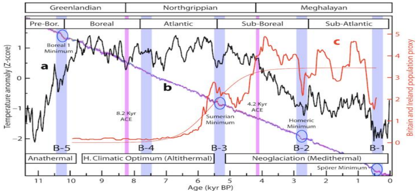
Figure 12d. The Bray 2500-yr solar and Holocene climate cycle. Holocene subdivisions are labelled with the stratigraphic subdivisions on top and biological subdivisions below, showing a 2500-yr spacing (after Ammann & Fyfe 2014)
