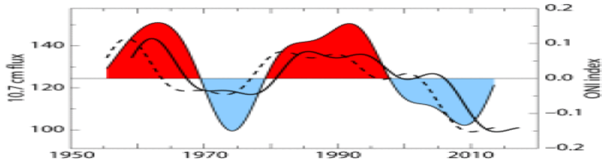
Figure 15a. Gaussian smoothed 1950-2018 Oceanic Niño Index (black line delimiting red and blue areas, right scale), and Gaussian smoothed 1950-2018 10.7 cm solar flux, a proxy for solar activity (thick dashed line, left scale).
