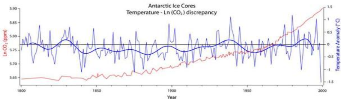
Figure 22. Temperature (blue) and CO 2 curve (red) from Antarctic Ice Cores Revised 800 kyr CO 2 Data (to 2001). Source: NOAA, contributed by Bereiter et al., (2015); and from NOAA annual mean CO 2 data (2002–2017). Temperature curve (blue) for the past 200 years from 5 high resolution Antarctic ice cores. Source: Schneider et al. (2006).
