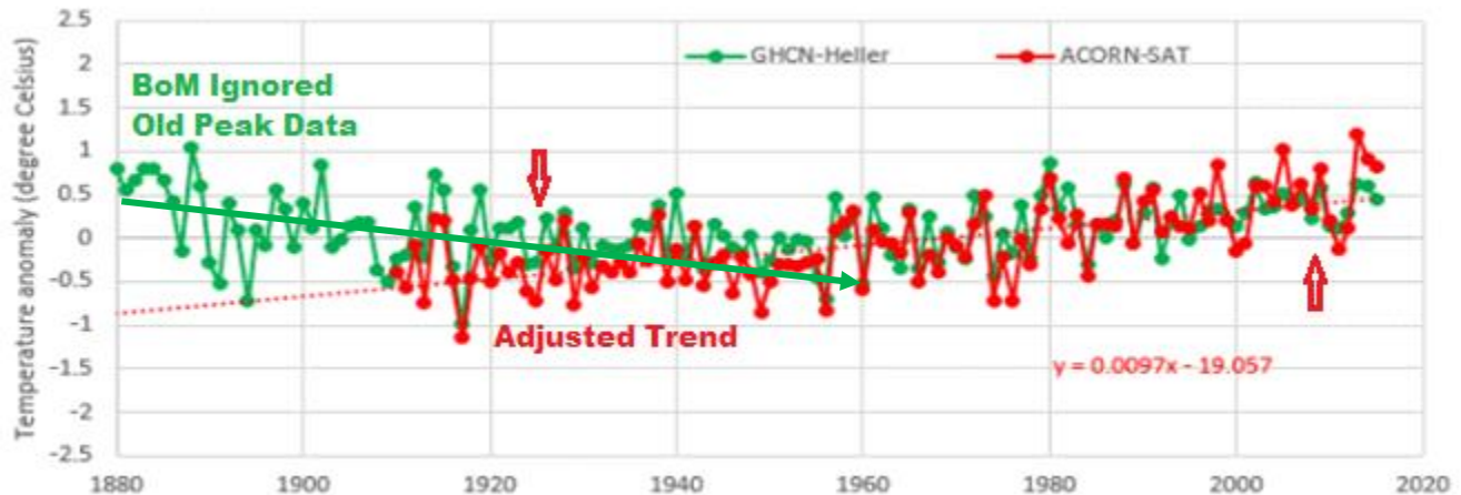
Figure 25b. Independent reanalysis showing Australian temperature maximums 1880-2015. Roberts (2016)
