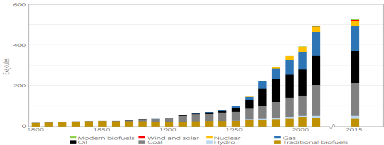
Figure 31. Composition of World total Primary Energy 1800 – 2015 After Smil 2020
