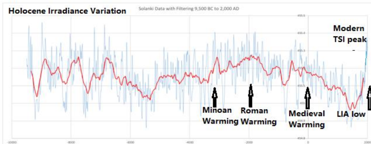
Figure 12c Solar TSI Oscillations during the Holocene. After Steinhilber et al. 2009; Vieira et al. 2011
