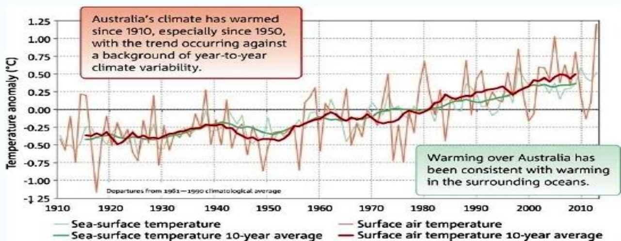
Figure 25a. Australian annual average sea and land temperatures 1910-2013 from a 2016 CSIRO presentation
