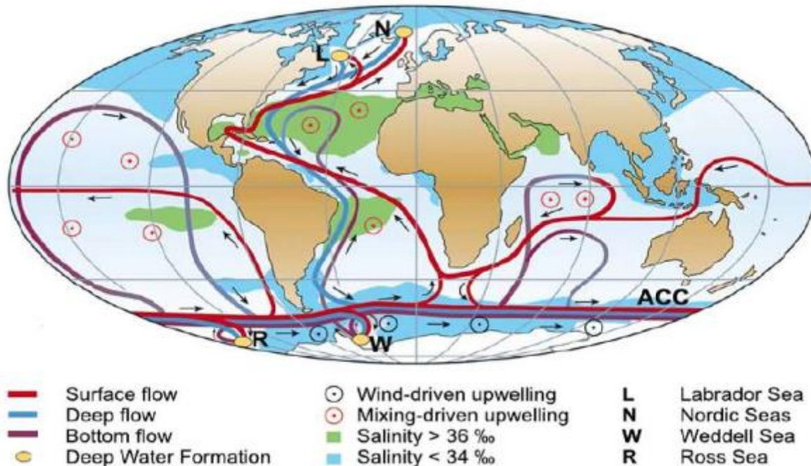
Figure 13a. Schematic of ocean currents associated with the global Meridional Overturning Circulation (MOC). With special focus on the Atlantic section of the flow (AMOC), where warm and saline waters flow northward from the Southern Ocean into the Labrador and Nordic Seas via the Gulf Stream. Kuhlbrodt et al. (2007).
