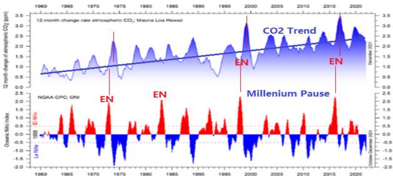
Figure 5b. NOAA data on El Niño-La Niña events since 1960 and Mauna Loa CO 2 levels, after Humlum 2020.
