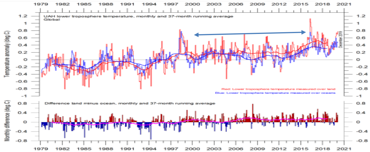
Figure 16c: UAH Lower troposphere temperatures: over land and ocean. Global monthly average temperature since 1979 measured by satellite over land and oceans, shown in red and blue, respectively, The thin lines represent the monthly average, and the thick line nearly corresponding to a running 3-year average. The blue arrows show the Pause.
