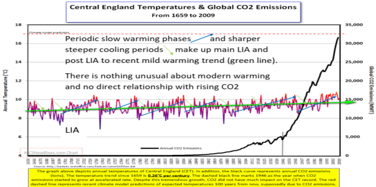
Figure 6. Historical cyclic Central England temperature data and atmospheric CO2.
