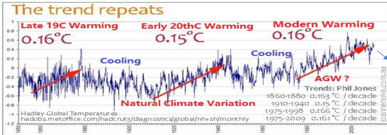
Figure 29. Global Temperature's repeating trends post 1850. After HadCRUT and Jones 2015.
