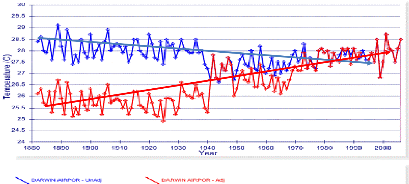
Figure 27. Comparison of Adjusted and Unadjusted (blue) Temperature Data for Darwin, Australia
