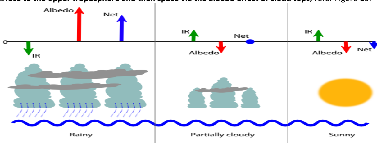
Figure 10: Conceptual model of typical variations of IR, albedo and net (IR + albedo) associated with three different areas of rain and cloud for periods of increased precipitation.
