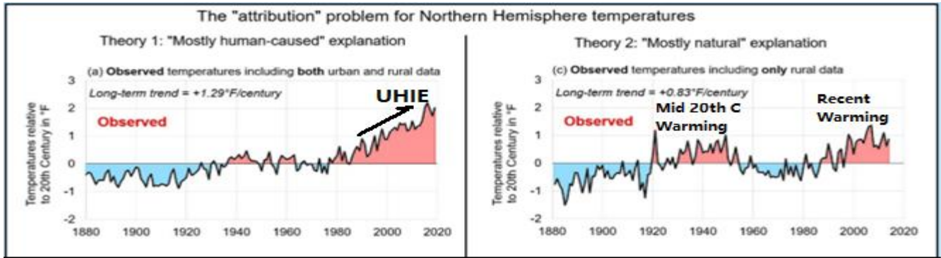
Figure 8c. USHCN US Historical temperature data comparing rural sites (right) and urban sites with UHIE. The above data shows the combined temperature record for all sites emphasises the modern UHIE warming trend from 1980 on the left. Whilst on the right the rural only sites shown much stronger relative warming in the first half of the 20 th Century from 1925-1950, cooling to 1980 then stronger warming peaking at 2010 with slow cooling to 2020. This rural data compares well with the UAH satellite data, thus highlighting the UHIE problem.
