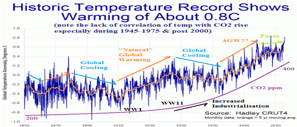
Figure 4. Original UK HadCRUT global temp data and CO2 rising trend. (Overall temp trend is 0.47C/century). This data shows the cyclic nature of post LIA warming over 165 years, which up to 1975 climatologists say is
