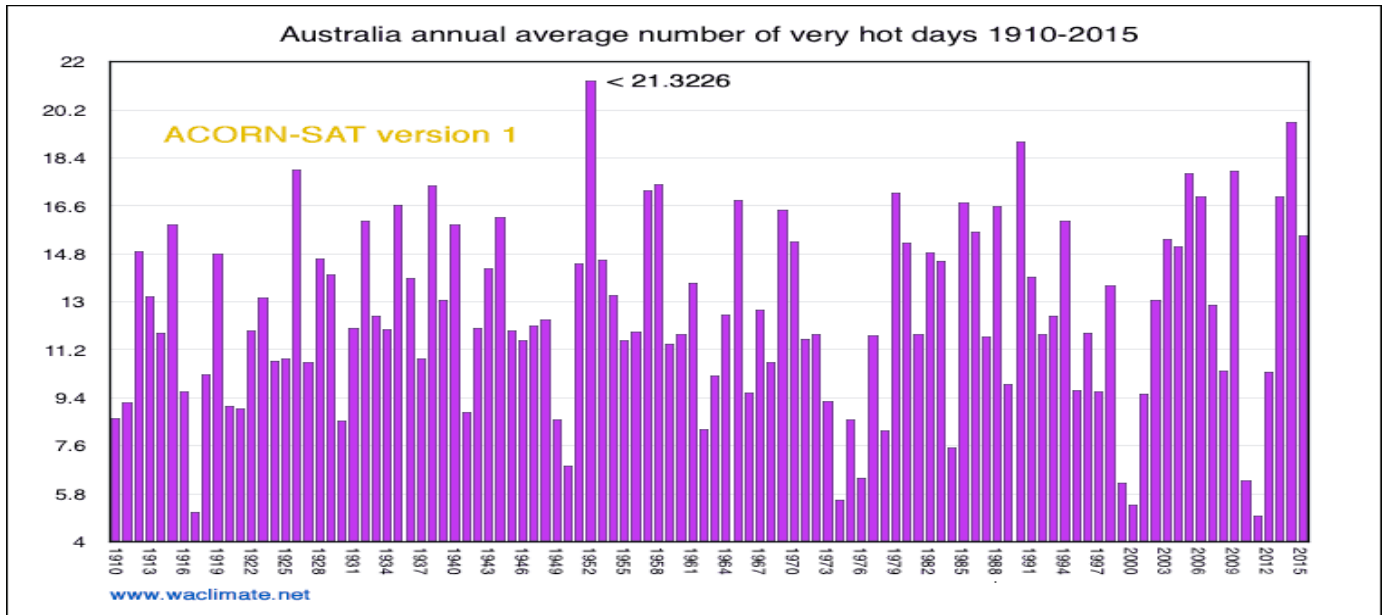
Figure 26. The BoM ACORN 1 & 2 dataset changes to Australia's temperature records 1910-2018
