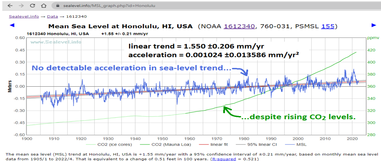
Figure 16b. Honolulu mean sea level over the last 117 years, showing no impact by CO2 (after NOAA)
