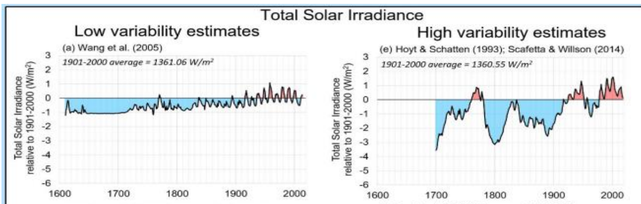
Figure 12a. Historical Total Solar Irradiance Low and High Variation estimates
