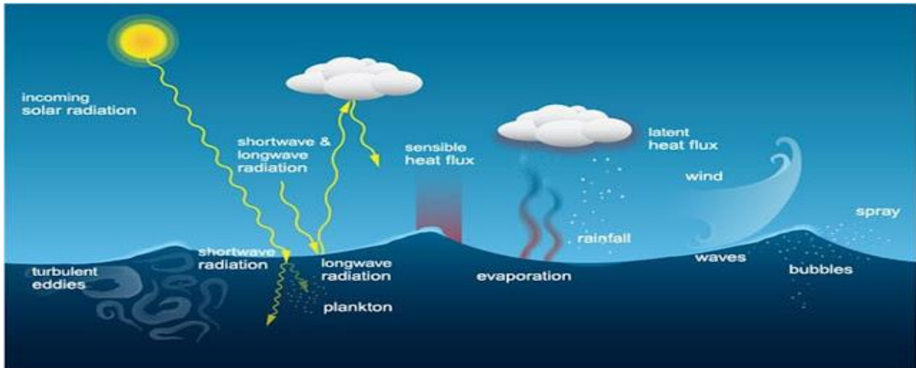
Figure 10a. Schematic showing solar radiation, the Hydrological cycle and latent heat flux
