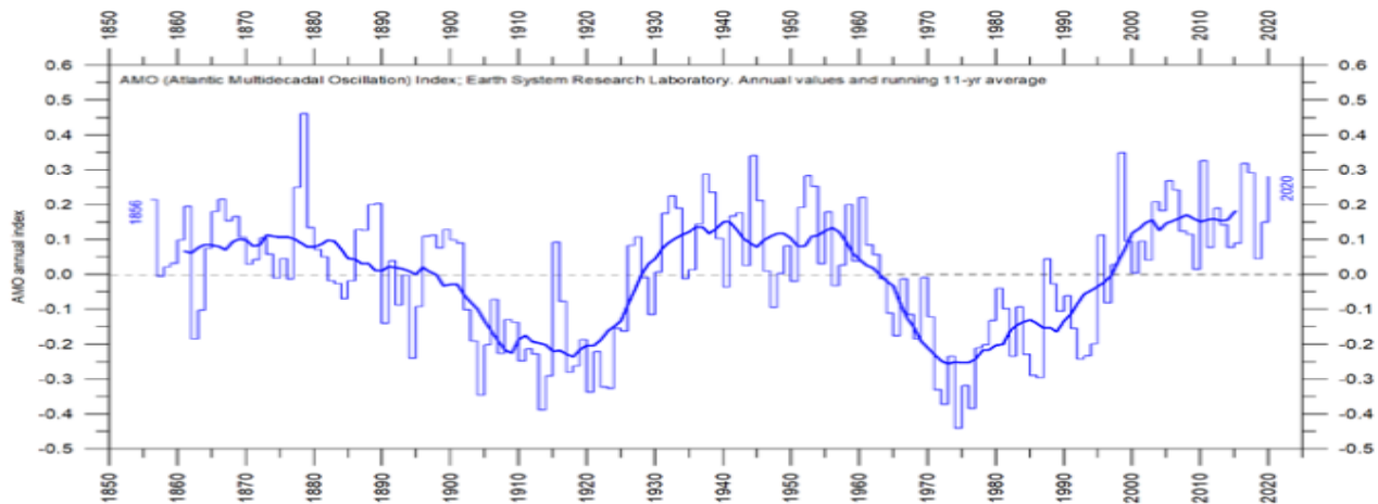
Figure 14a: Annual values 1855-2020 of the Atlantic Multidecadal Oscillation from Humlum 2020
