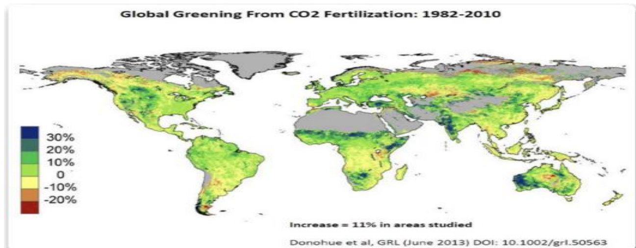
Figure 24. Global greening due to CO 2 fertilization 1982 to 2010
