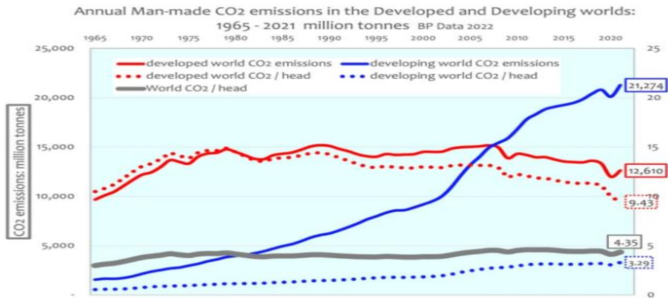
Figure 30. CO2 Emissions trends in Developed and Undeveloped Nations, from BP data 2022.
