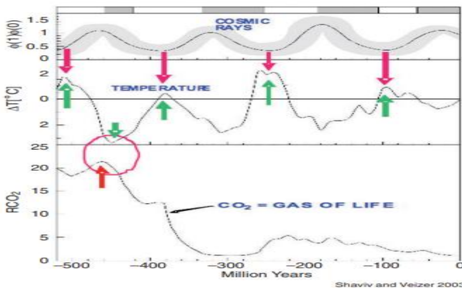
Figure 18b. Phanerozoic temperature fluctuations correspond with the cosmic ray flux and not CO 2 .
