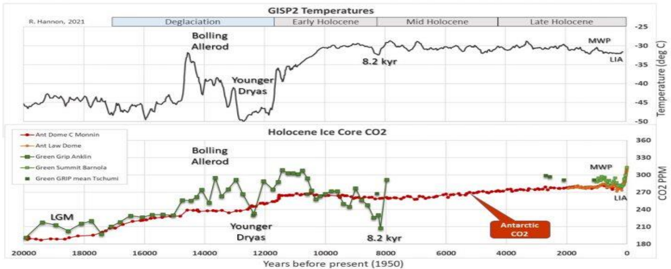
Figure 20a. Greenland ice core T and CO 2 compared to Antarctic ice CO 2 over 20,000 years since last glacial. From Hannon 2021: GISP2 ice core temperatures derived from oxygen isotopes by Alley, 2004. Greenland ice core CO 2 compared to the Antarctic ice core CO 2 composite (red line).
