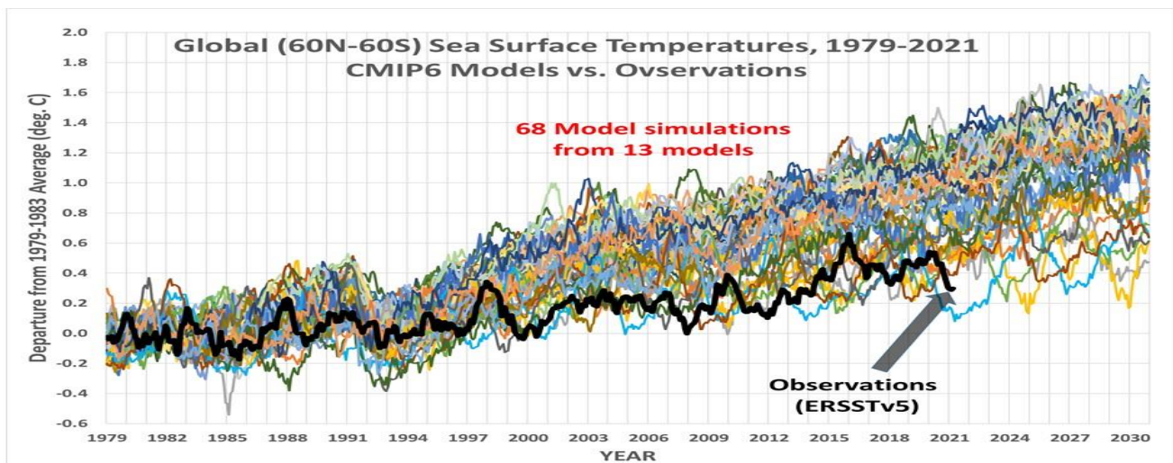
Figure 15c. Ocean temperature satellite observations and model results.
