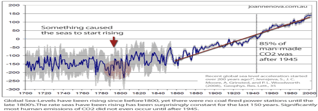
Figure 16a. Global sea levels over the last 300 years, showing the lack of impact by AGW since WW2.
