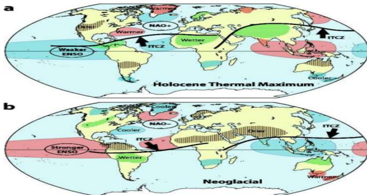
Figure 21. The transition from a) Holocene Climatic Optimum to b) Neoglaciatio.
