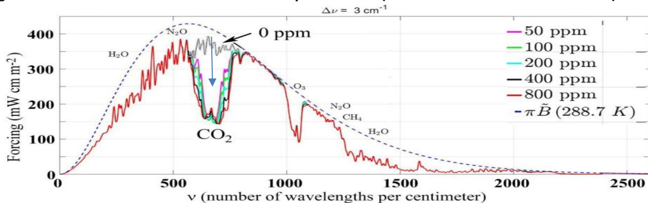
Figure 11a. A direct estimate of Climate Sensitivity to \text{CO}_2 -ECS. (after Rotter 2021 in Fabius Maximus)
