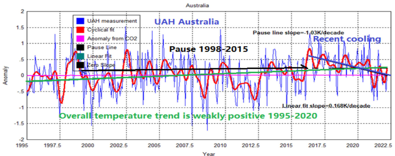
Figure 28. Australian UAH data 1995-2022.
