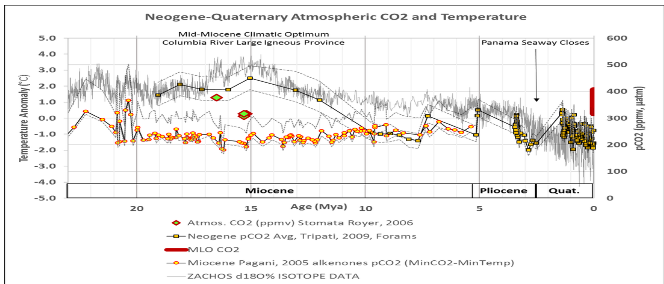
Figure 19. Miocene-Quaternary Global temperature and carbon dioxide levels
