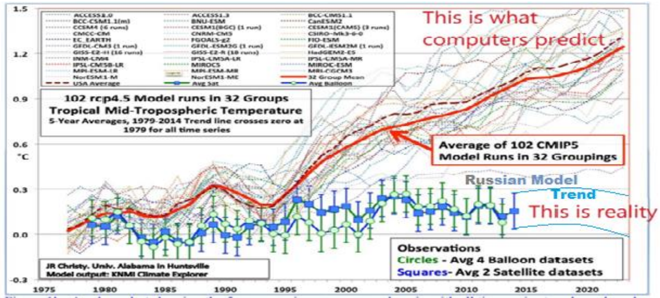
Figure 9b. CMIP5 model projections and modern observation data, after Christie (2018)
