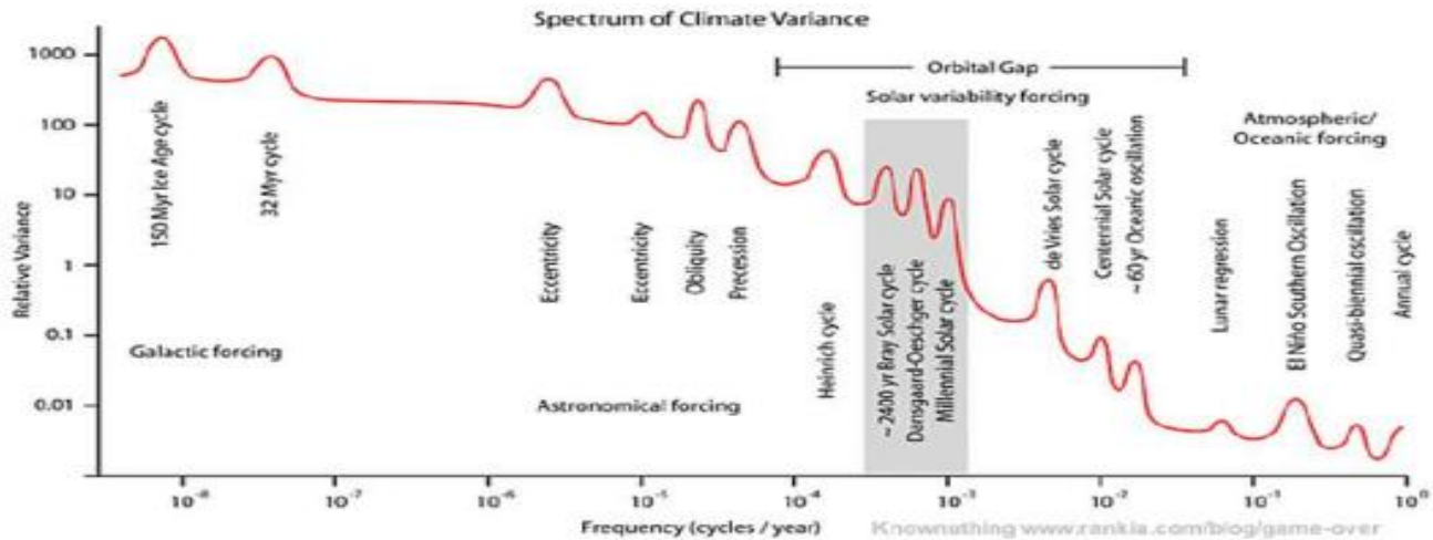
Figure 17. A periodogram shows how periodicities (either of orbital or solar origin) dominate climate change at all temporal scales, adapted by Javier (2017).
