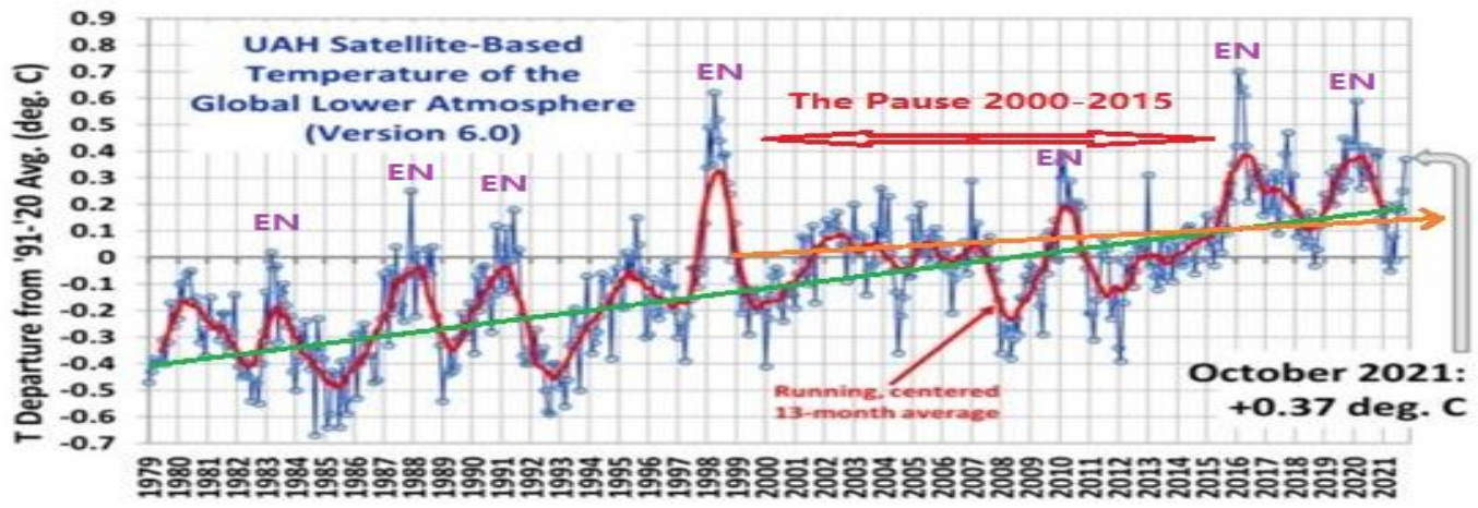
Figure 3. The satellite linear warming trend (green) since January, 1979 has weakened from +0.14 to +0.13 C /decade (+0.12 C/dec over the global-averaged oceans, and +0.18 C/dec over global-averaged land).
