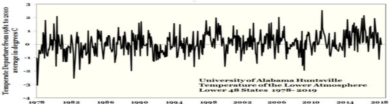
Figure 7. UAH satellite air temperatures showing +/-2C variation for the contiguous United States of America.
