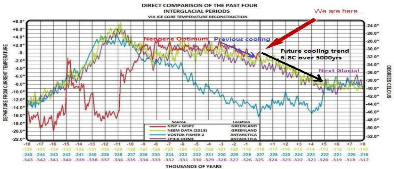
Figure 23. Interglacial temperature trends from Ice Cores, indicating likely future cooling trend.
