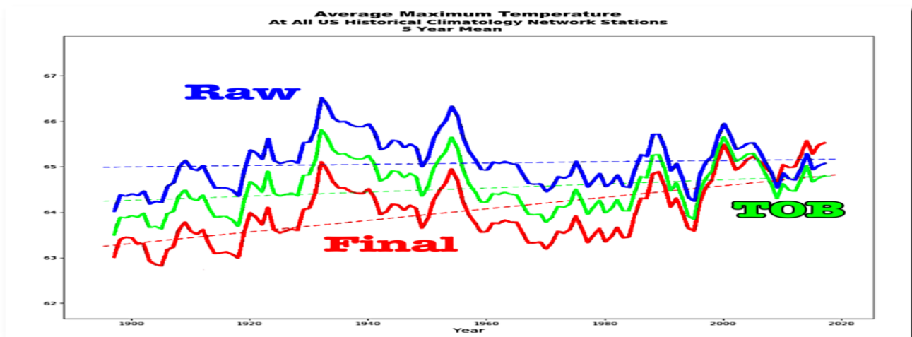
Figure 8b. NOAA USA Temperature Data Adjustments. Temperatures prior to 1980 are cooled more than 1C degree, and recent temperatures are warmed nearly 1 degree. This is extreme data manipulation!
