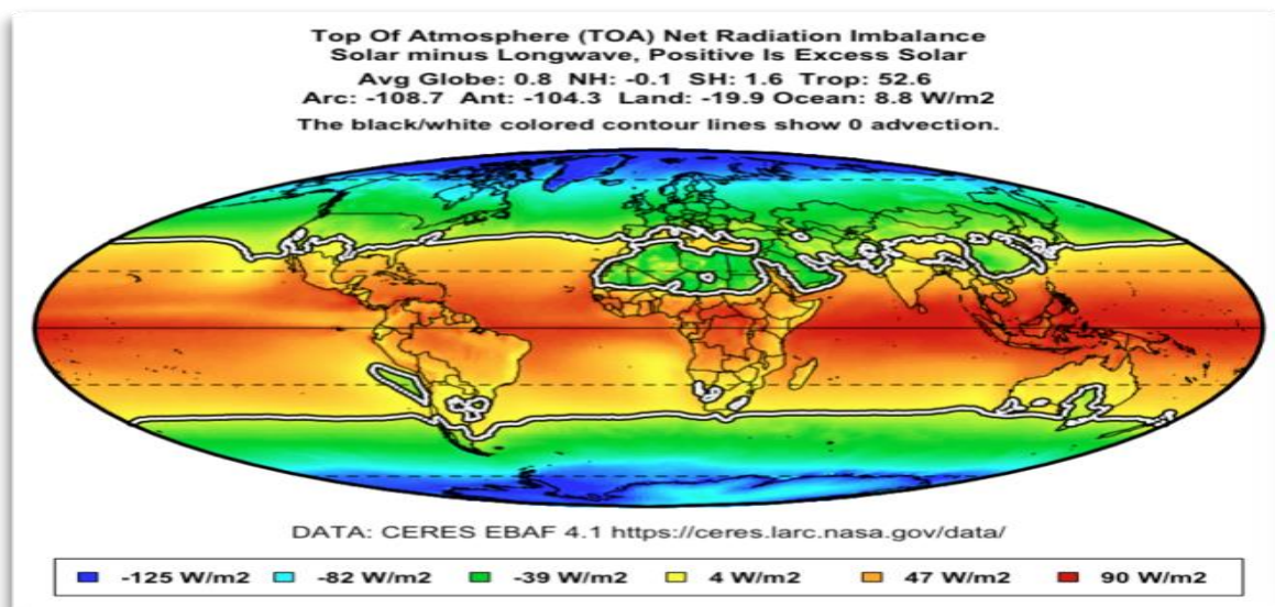
Figure 12b. Top-of-atmosphere (TOA) average radiation balance, 2000-2021, Ceres data. After Eschenbach 2021.
