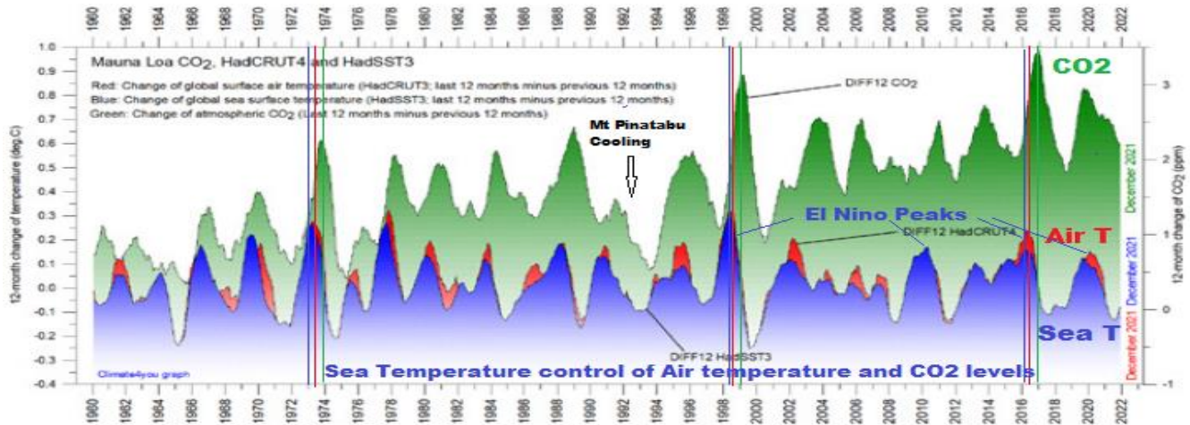
Figure 1. UK HadCRUT global CO2 and sea/air temperatures, after Humlum 2020.
